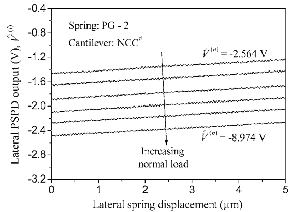
FIG. 5. D-LFC data of the lateral PSPD output showing a linear dependence on the lateral spring displacement under incremental normal loads (a) for the NCD d cantilever-bead and (b) for the NCC d cantilever-tip assemblies.
