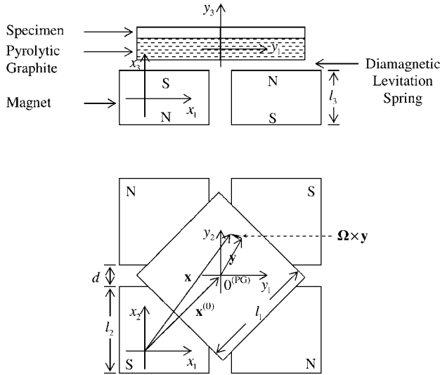
FIG. 2. Diamagnetic levitation load cell of the D-LFC: (x_1, x_2, x_3) are the magnet coordinates, (y_1, y_2, y_3) the levitated-mass coordinates, and \Omega the rotation vector of the levitated mass.
