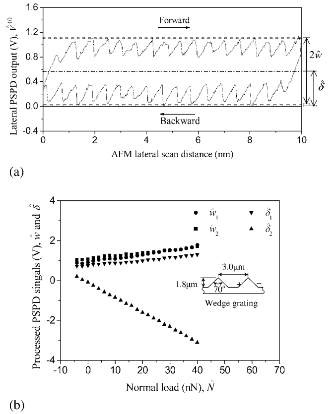
FIG. 6. (a) A friction loop of a contact B tip sliding on a mica surface: \hat{w} and \hat{\delta} denote the half-width and the central-value offset of the loop. (b) W-LFC data of \hat{w} and \hat{\delta} , which depend on the normal load for the NCC* tip sliding on the two different slopes of a wedge.
