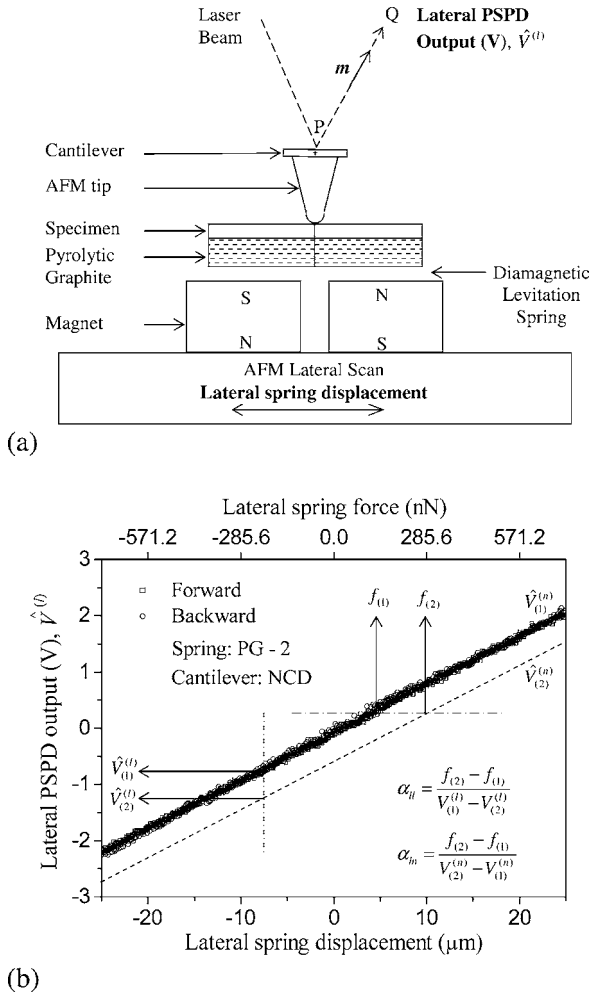
FIG. 4. (a) A schematic of the D-LFC. (b) A diagram showing the D-LFC principles for measuring the force constants \alpha_{||} and \alpha_{\perp} : the data set was collected with the PG-2 diamagnetic spring for the NCD AFM cantilever-bead assembly.
